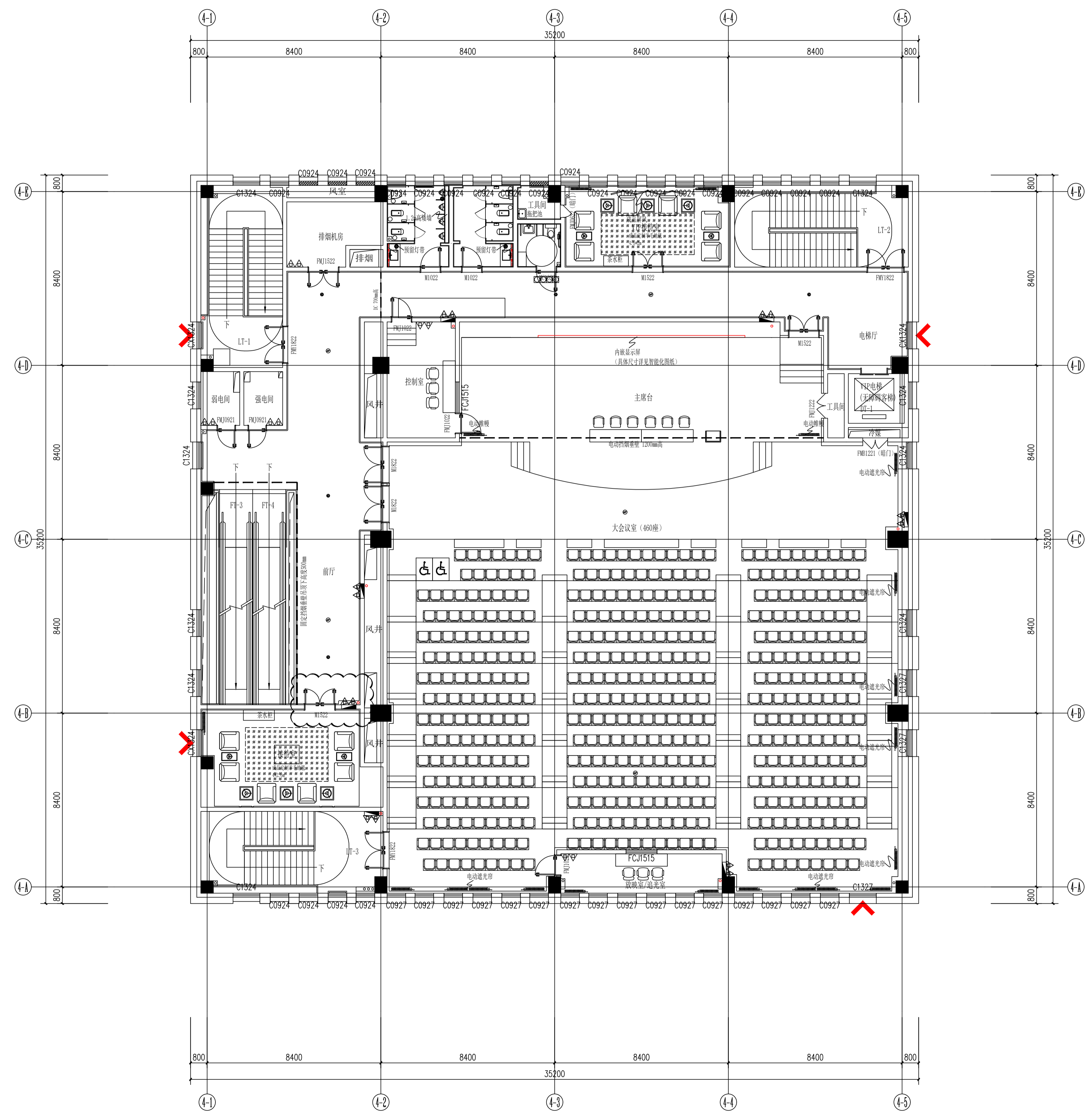
FF 3F FIXTURE/FURNISHING PLAN 三层平面布置图 SCALE: 1/100
