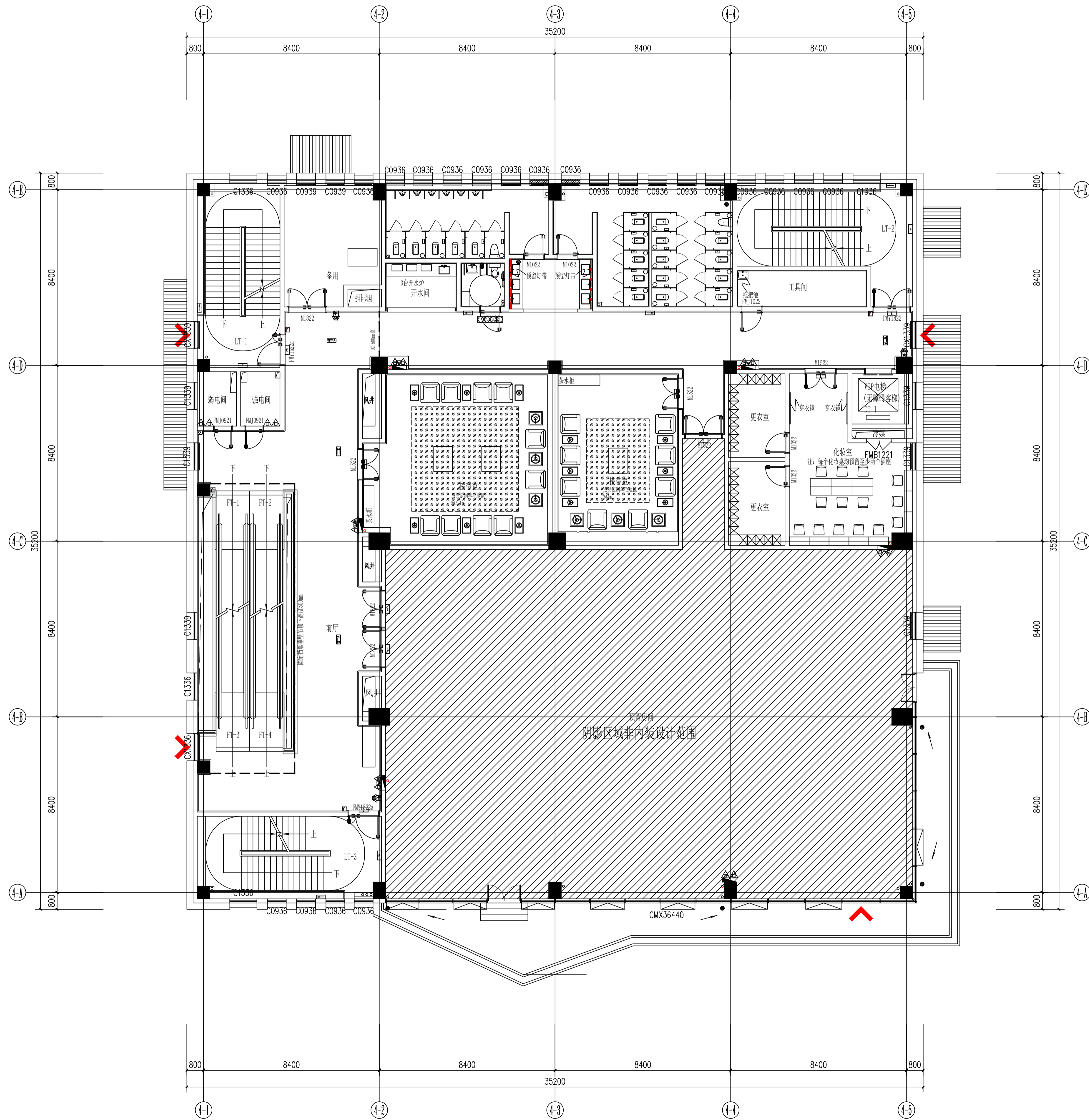
FF 2F FIXTURE/FURNISHING PLAN 二层平面布置图 SCALE: 1/100
