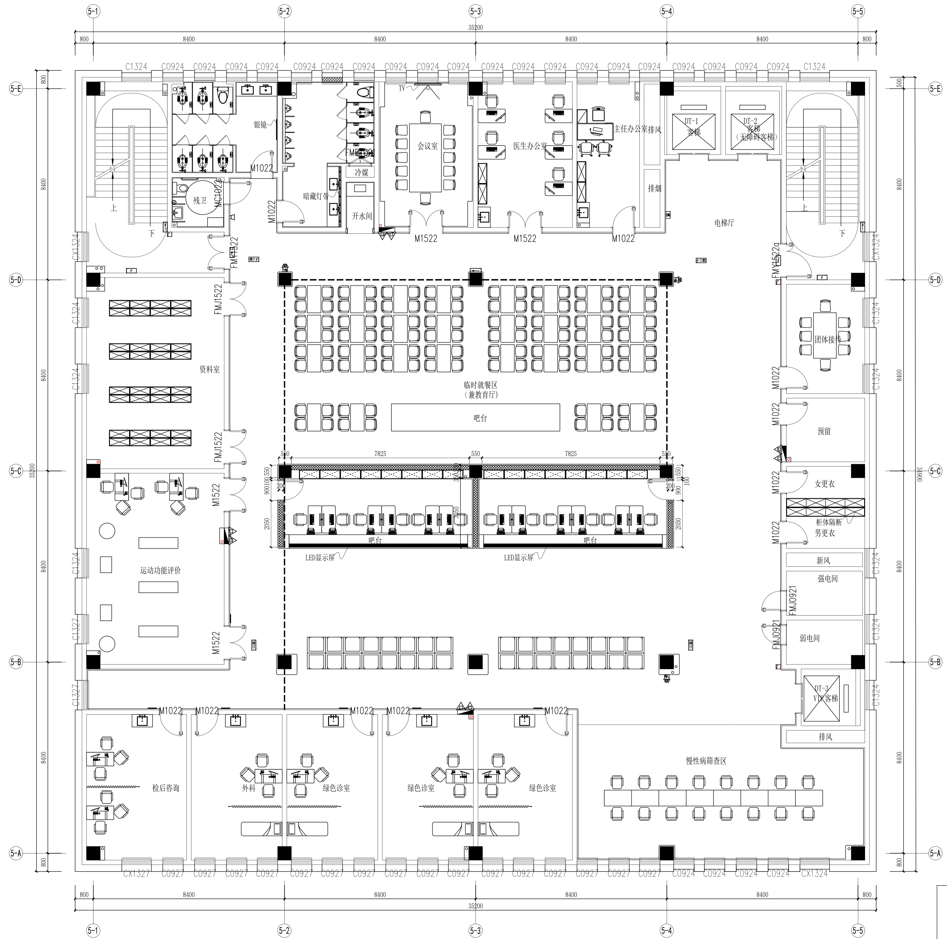
FF 3F FIXTURE/FURNISHING PLAN 三层平面布置图 SCALE: 1/75
