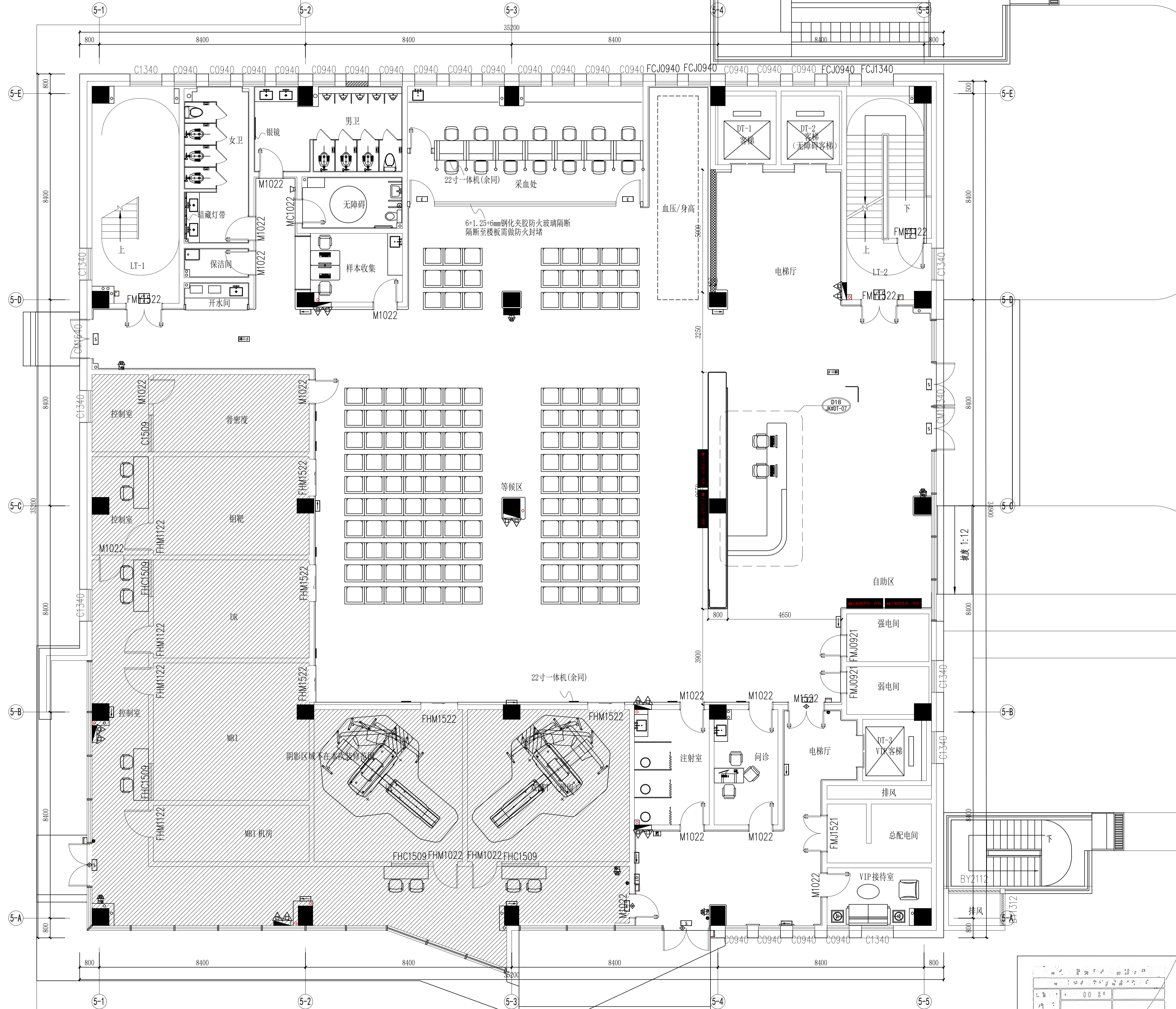
1F FIXTURE/FURNISHING PLAN 一层平面布置图 SCALE: 1/75
