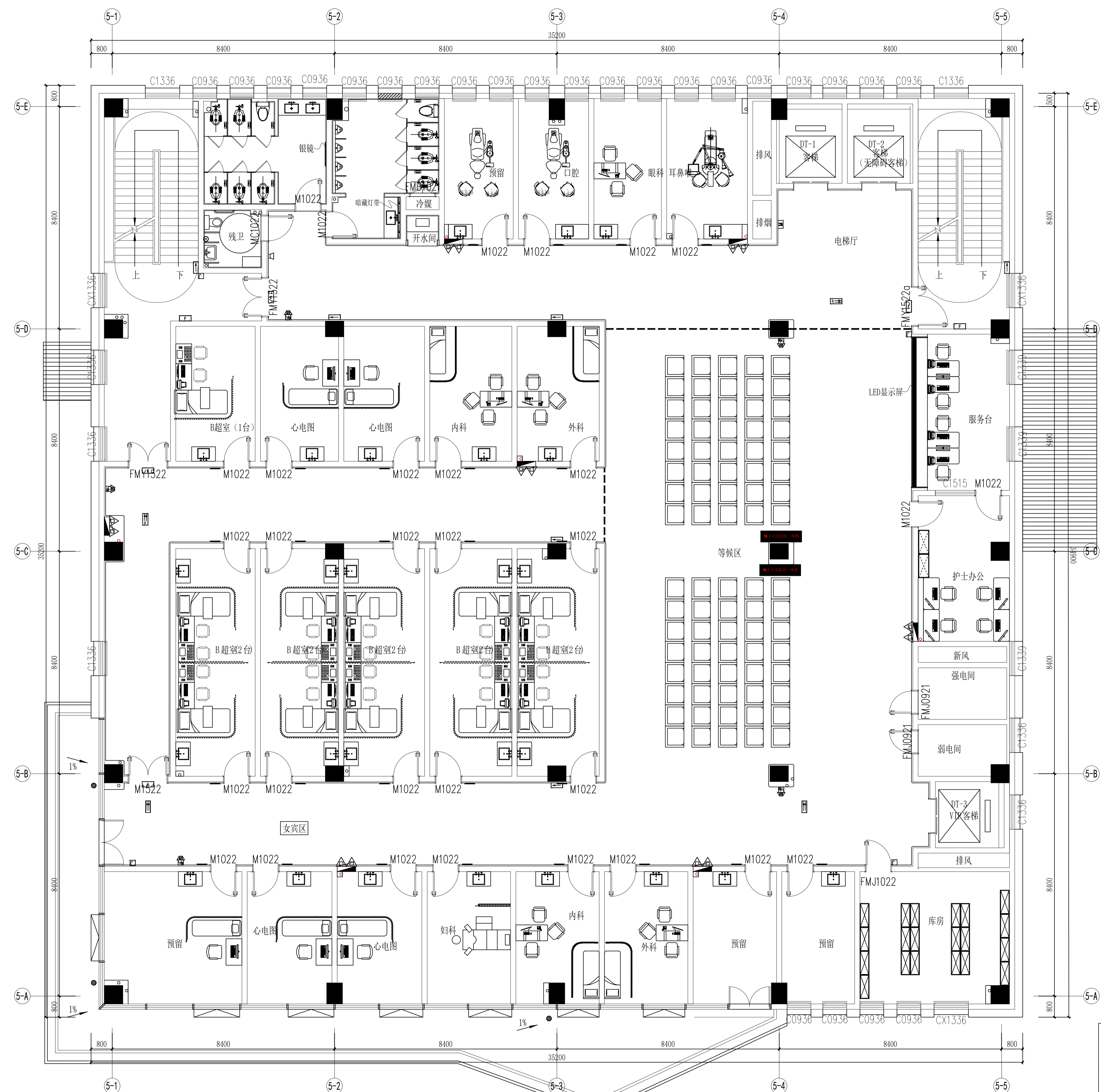
2F FIXTURE/FURNISHING PLAN 二层平面布置图 SCALE: 1/75
